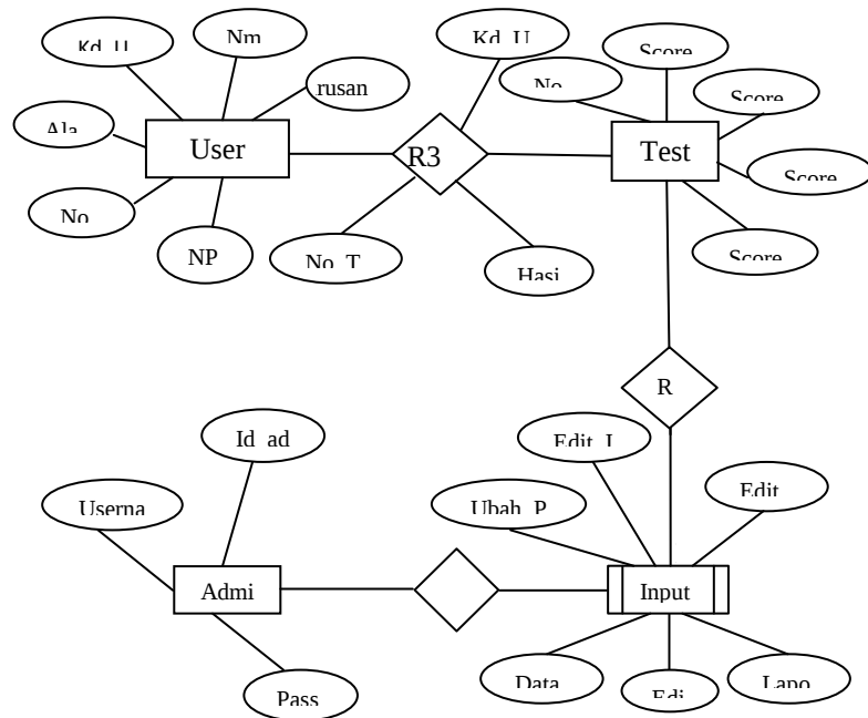
Gambar 2. ER-Diagram
