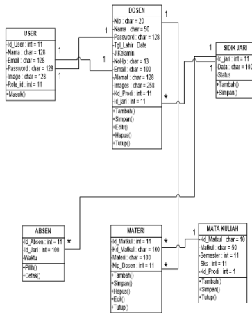
Gambar 2. Class Diagram
