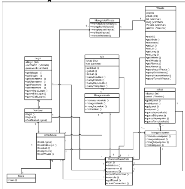
Gambar 8. Class Diagram
