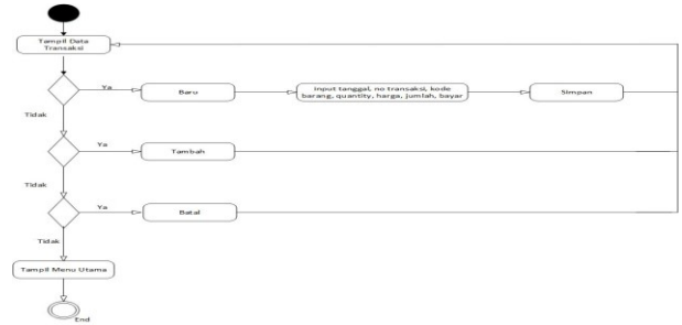
Gambar 7. Activity Diagram Transaksi
