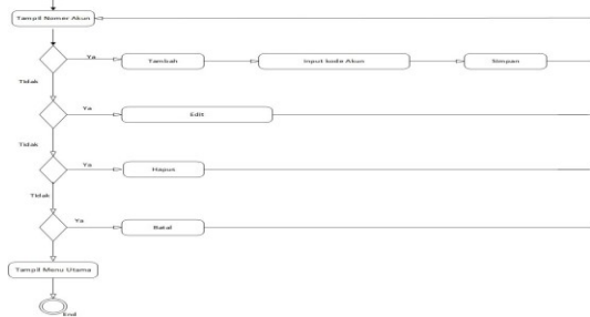
Gambar 4. Activity Diagram Nomor Akun
