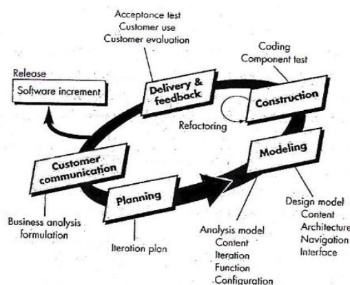
Gambar 3.1 Ilustrasi model Web Engineering
