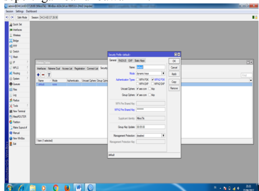
Gambar 21. Tampilan security profile
